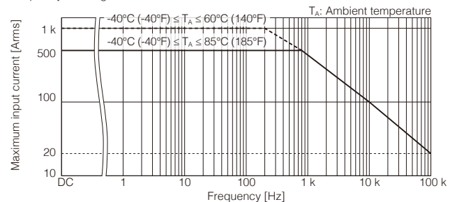
Frequency derating
