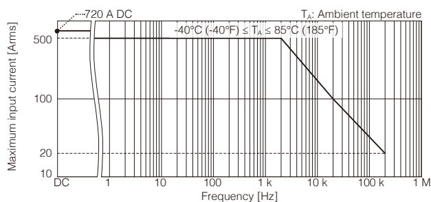
Frequency derating
