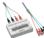
TEST FIXTURE 9261-10 Cable length 1 m (3.28 ft), DC to 8 MHz, impedance characteristics of 50 Ω, 4-terminal pair configuration, measurable conductor diameter: ø0.3 mm (0.01 in) to 1.5 mm (0.06 in)
