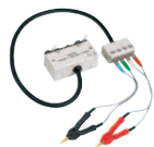
FOUR-TERMINAL PROBE L2000 Cable length 1 m (3.28 ft), DC to 8 MHz, impedance characteristics of 50 Ω, 4-terminal pair configuration, measurable conductor diameter: ø0.3 mm (0.01 in) to 5 mm (0.20 in)
